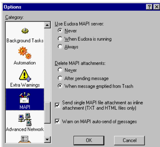
MAPI options window
